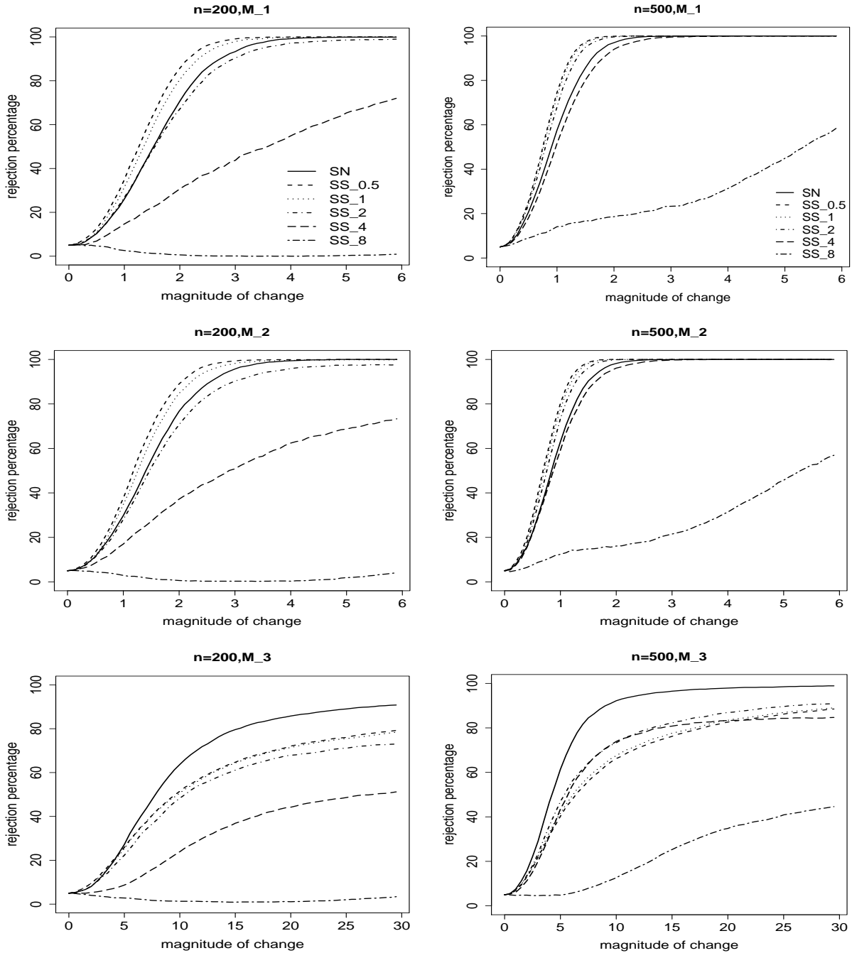
Figure 3: Size-adjusted power curve in detecting a change point in median for the models M_1 , M_2 and M_3 . Here SN denotes the SN-based method and SS_c denotes the subsampling method with the subsampling width being cn^{1/3} . Sample size n = 200 (left panel) and 500 (right panel).
