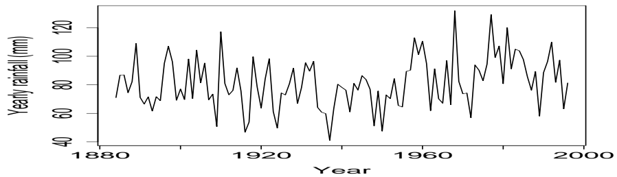
Figure 5: Argentina rainfall data: yearly rainfall (milimeters) in Argentina from 1884 to 1996
