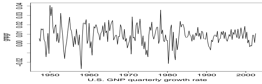
Figure 4: Quarterly U.S. GNP growth rate from 1947(1) to 2002(3)
