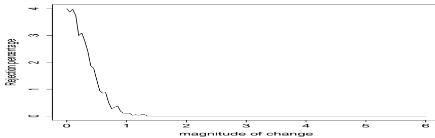
Figure 1: The empirical rejection percentage of the naive SN-based test \widetilde{KS}_n under the alternative model (3).
